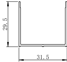
0833# wall profile
