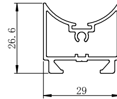
0834# hinge profile
